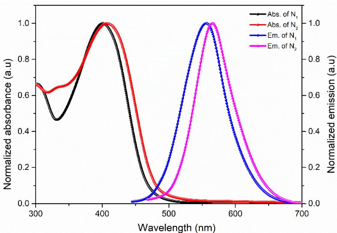
Figure 3. Intersection of UV-Vis absorption and fluorescence emission spectra of N 1-2 recorded in 10 -5 M DMF solution under ambient atmosphere
